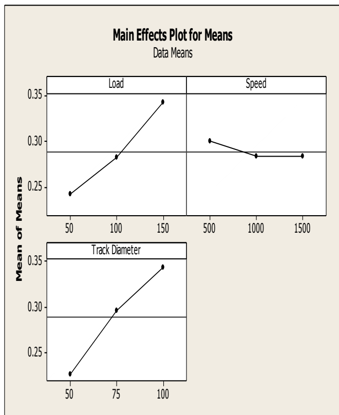
Fig 4.2 Main Effects Plot for Means– Weight Loss
