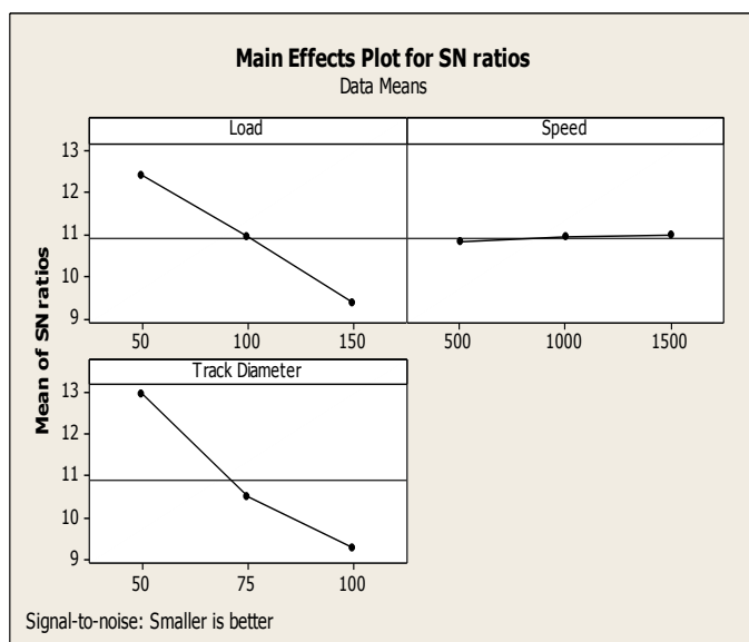
Fig 4.1 Main Effects Plot for S/N ratios – Weight Loss
