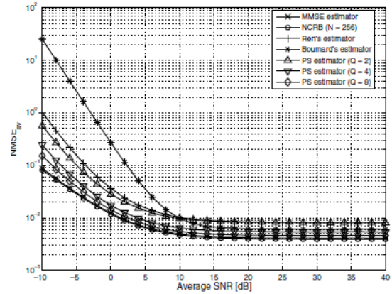
Fig. 4. NMSE vs Average SNR in AWGN channel
