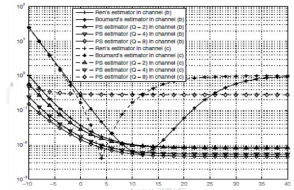
Fig. 5. NMSE vs Average SNR in Rayleigh and Rician channels
