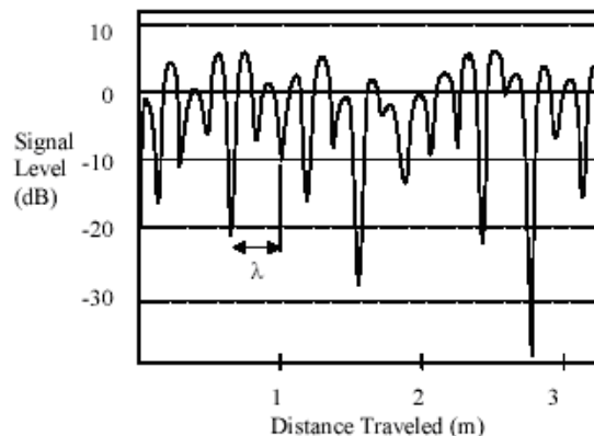
Fig. 2. Typical Rayleigh fading when the mobile unit is moving
