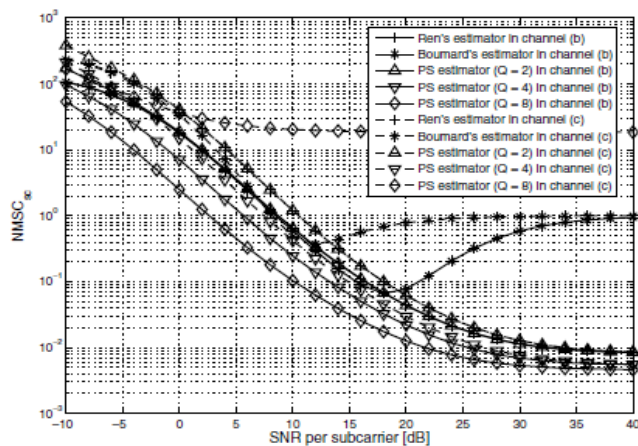
Fig. 6. NMSE vs Average SNR per sub carrier in Rayleigh and Rician channels
