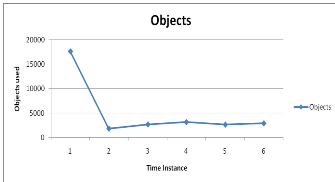
Fig. 1 Time taken by Node to initialize by objects.
