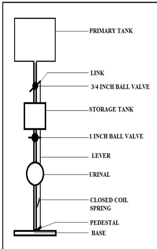
Fig. 2 Front view of the Automatic urinal flushing system
