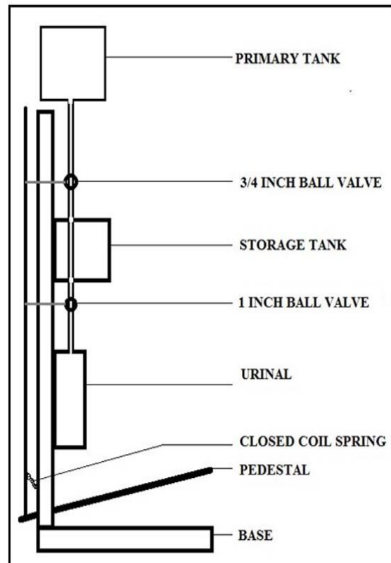
Fig. 1 Side view of the Automatic urinal flushing system
