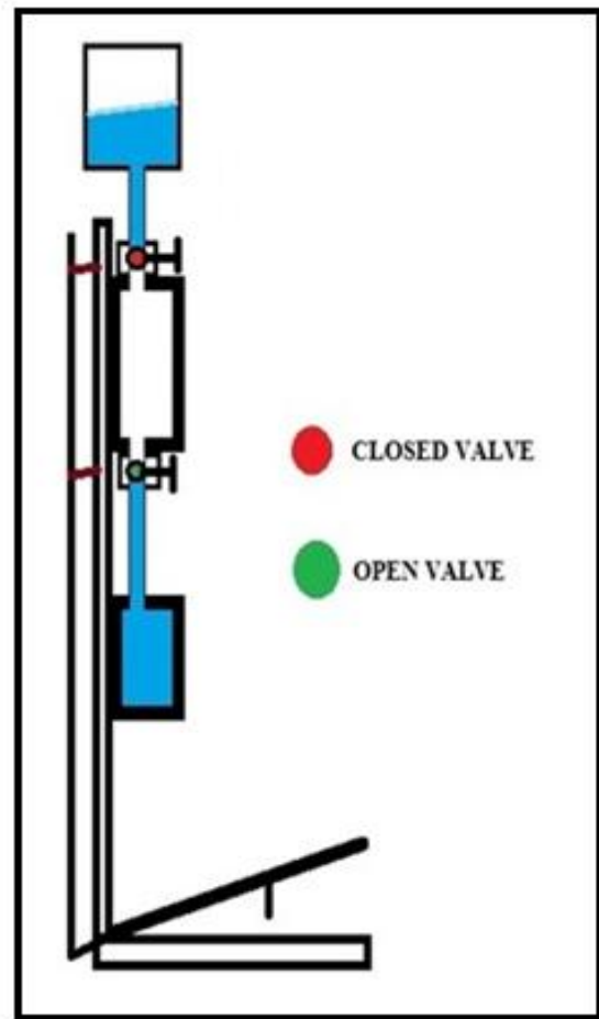
Fig. 5 Final stage of operation
