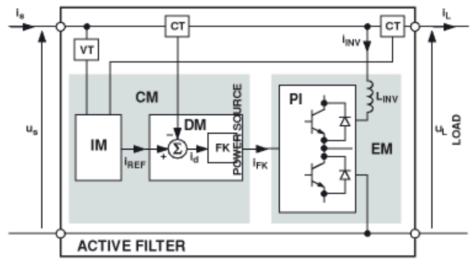
Fig.5 Active Filter Block Diagram
