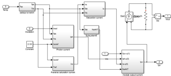
Fig.13 PV solar system
