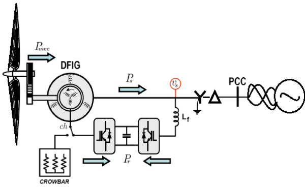
Fig.3 The doubly-fed induction generation
