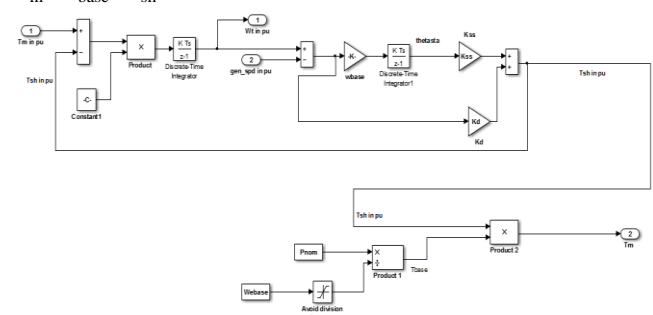
Fig.11 Drive train modelling
