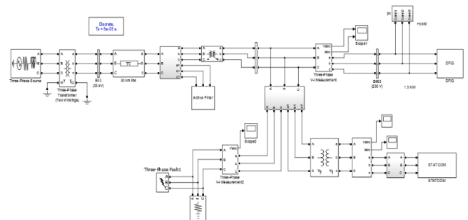
Fig.16 DFIG and STATCOM connected to grid
