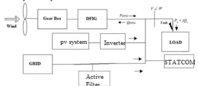
Fig.1 Hybrid System connected to the system with AF & STATCOM
