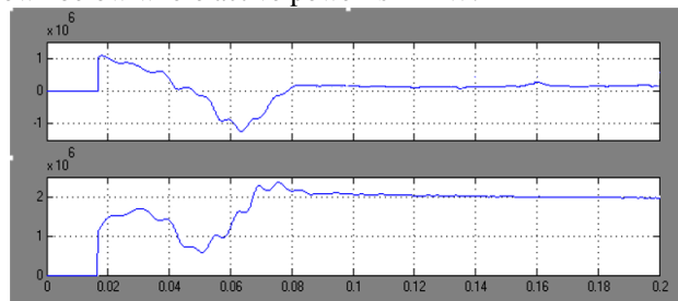
Fig.20 Reactive and a=Active power of DFIG
