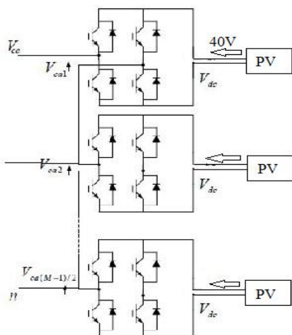
Fig.4 Three level STATCOM
