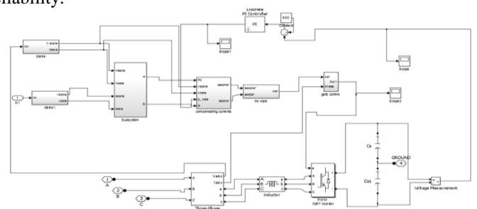
Fig.15 AF simulation model
