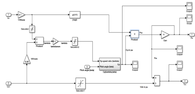
Fig.10 Wind turbine modelling
