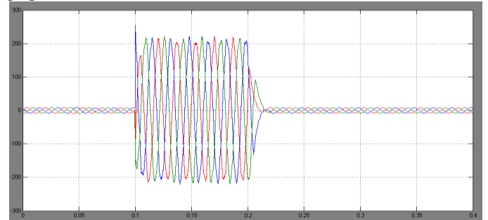
Fig.22 STATCOM injection voltage
