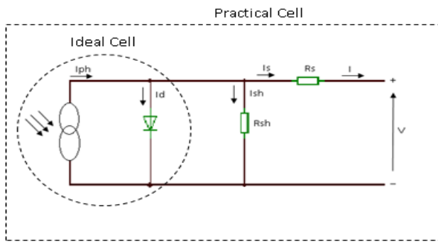
Fig.2 An ideal PV cell
