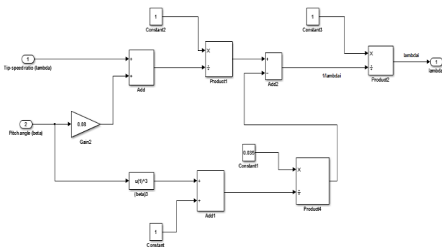
Fig.7 1/Lambda model
