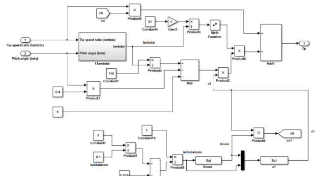
Fig.9 Cp Model
