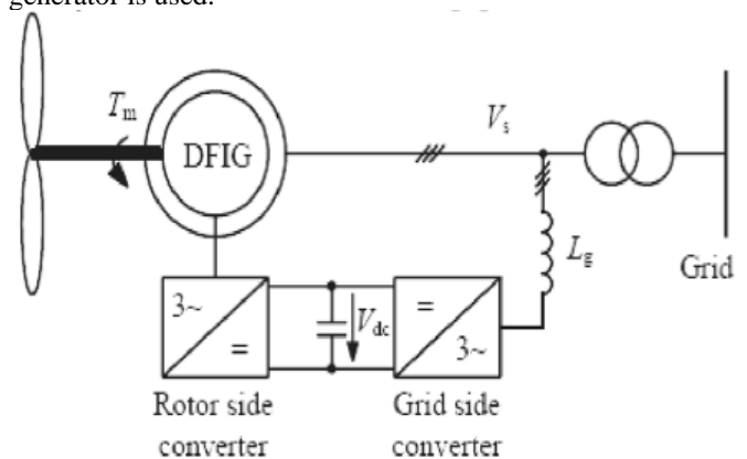
Fig.6 Wind Turbine DFIG
