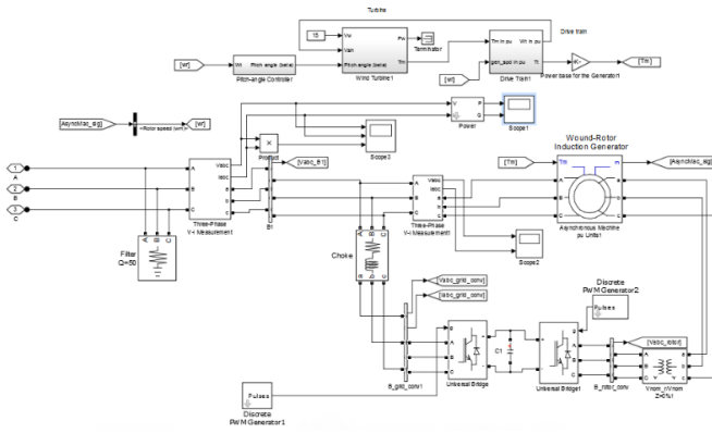
Fig.12 DFIG model
