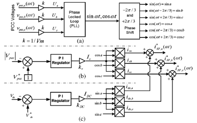
Fig.14 STATCOM controller
