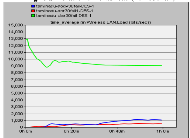
Fig 14 Simulation time v/s load (30 node fail)
