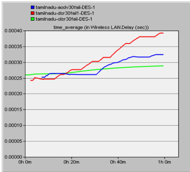
Fig 10 Simulation time v/s delay (30 node fail)
