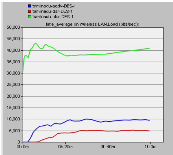
Fig 11 Simulation time v/s load (without node fail)
