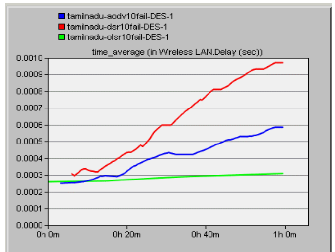
Fig 8 Simulation time v/s delay (10 node fail)
