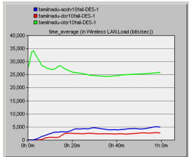
Fig 12 Simulation time v/s load (10 node fail)
