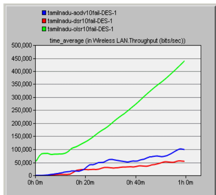
Fig 4 Simulation time v/s throughput (10 node fail)
