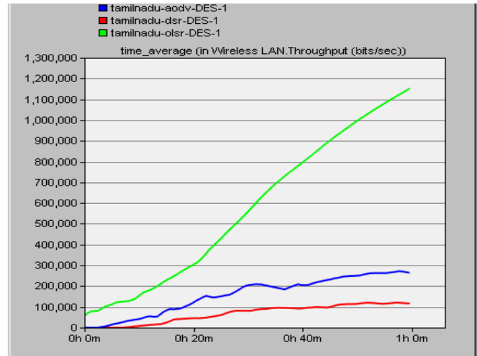
Fig 3 Simulation time v/s throughput (without node fail)
