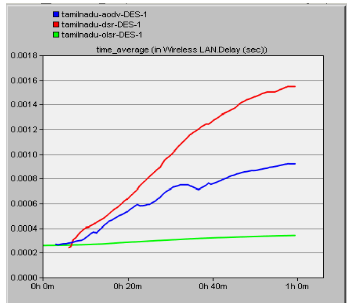
Fig 7 Simulation time v/s delay (without node fail)
