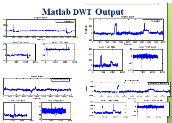
Image 2: DWT Signal
