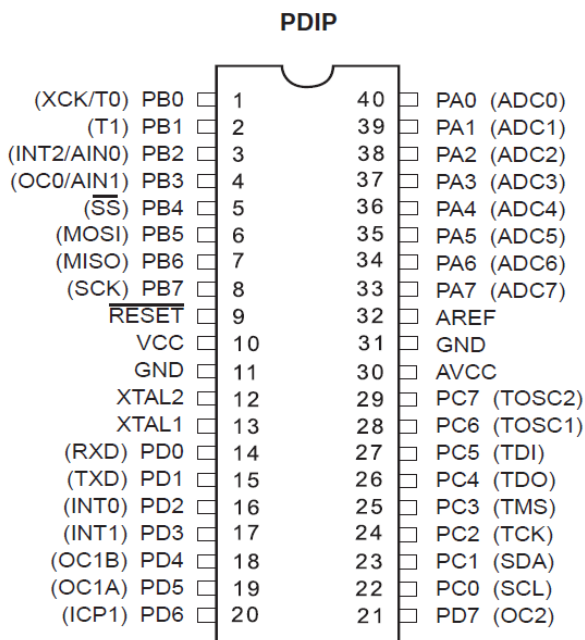
Figure 2: Pin configuration of ATmega32 (DIP)
