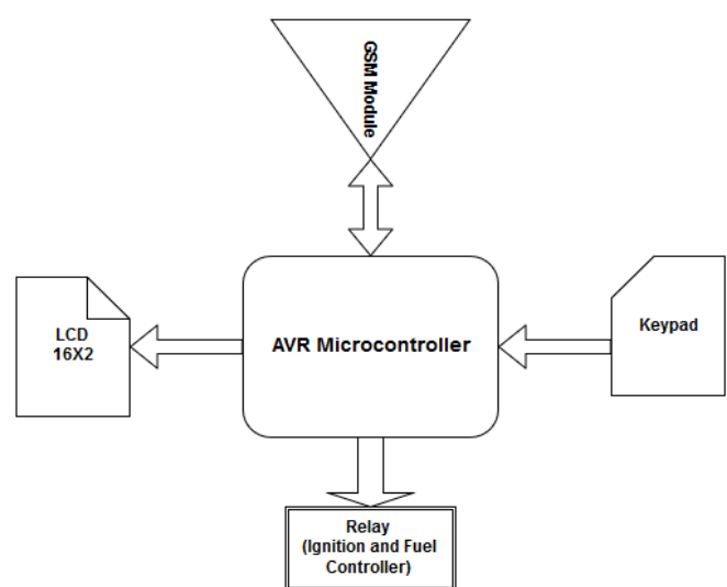
Figure 1: Block Diagram of the embedded system.
