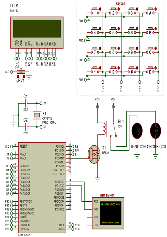
Figure 4: Simulation Schematic of the embedded system.
