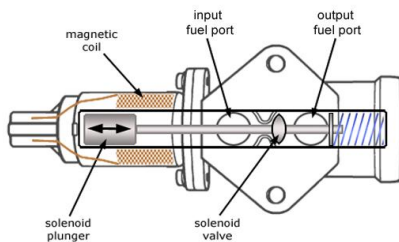
Figure 5: Choke coil in fuel injection system
