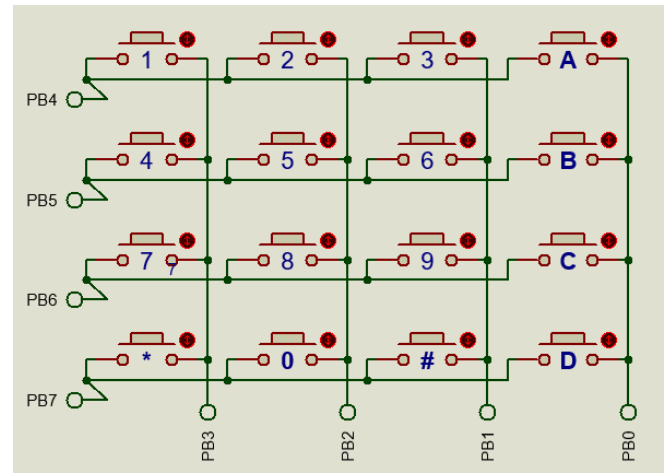
Figure 3: The designed keypad
