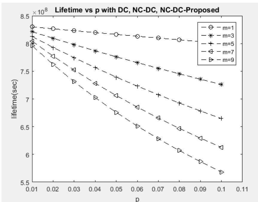
Fig. 5 Lifetime of Sensor Network using Adaptive Duty Cycle and Network Coding
