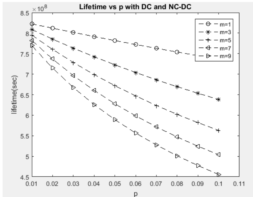
Fig. 5 Lifetime of Sensor Network using Random Duty Cycle
