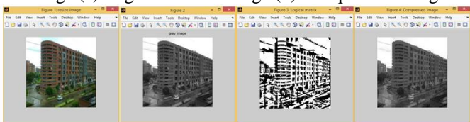
Figure 17: BTC-PF Algorithm applied on Mall Image of block size 16x16: (a) Original image of size 255*255 (b) Gray Image (c) Logical Matrix Image (d) Compressed Image
