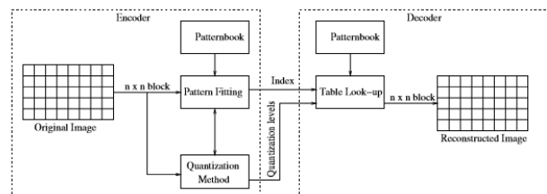
Figure 2: A schematic diagram of BTC-PF method.
