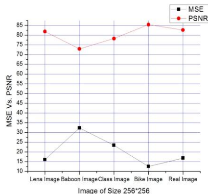
Figure 33: MSE Vs. PSNR for Gray Scale Image of Block Size 4x4
