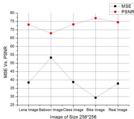
Figure 34: MSE Vs. PSNR for Gray Scale Image of Block Size 8x8
