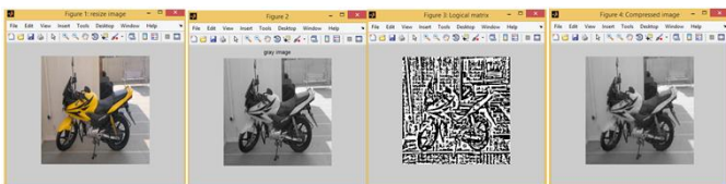
Figure 11: BTC-PF Algorithm applied on Bike Image of block size 8x8: (a) Original image of size 255*255 (b) Gray Image (c) Logical Matrix Image (d) Compressed Image
