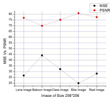
Figure 34: MSE Vs. PSNR for Gray Scale Image of Block Size 8x8
