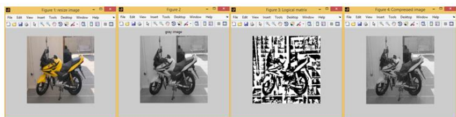
Figure 16: BTC-PF Algorithm applied on Bike Image of block size 16x16: (a) Original image of size 255*255 (b) Gray Image (c) Logical Matrix Image (d) Compressed Image
