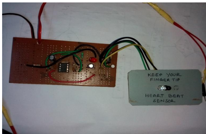
Fig 2. PCB connection of IR sensor
