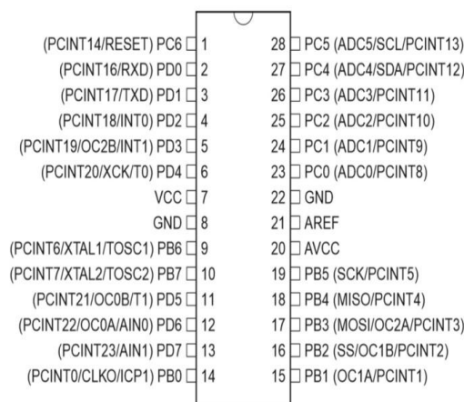
Fig 6. Pin diagram of Atmega328
