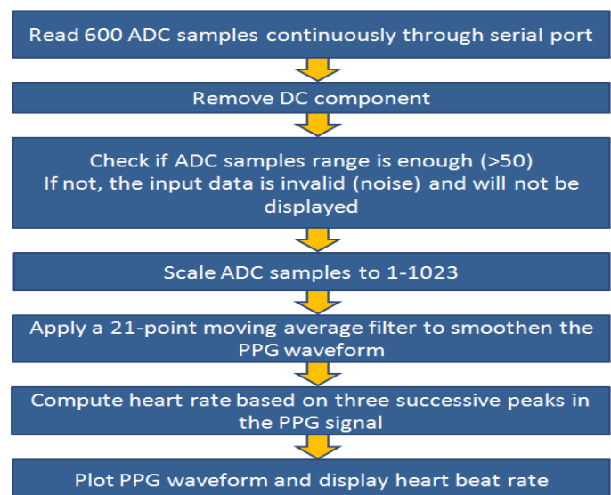
Fig 9.Flow chart for computing pulse rate
