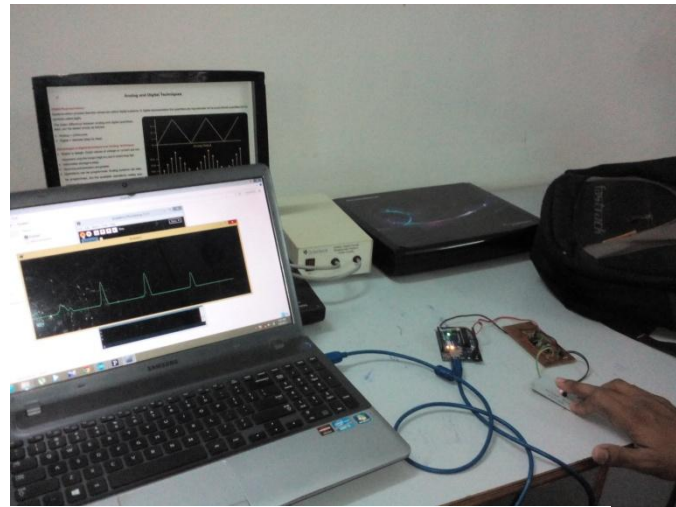
Fig7. PPG waveform and heart rate displayed on computer screen
