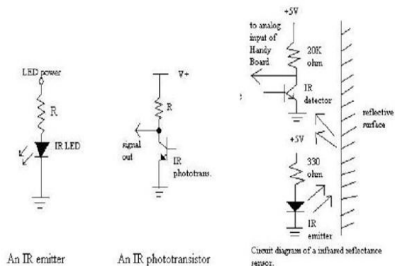
Fig 3. Working of IR sensor
