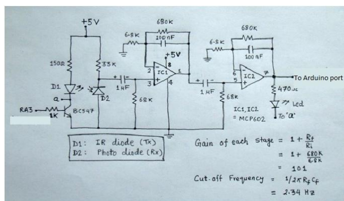
Fig1. Circuit diagram of sensor
