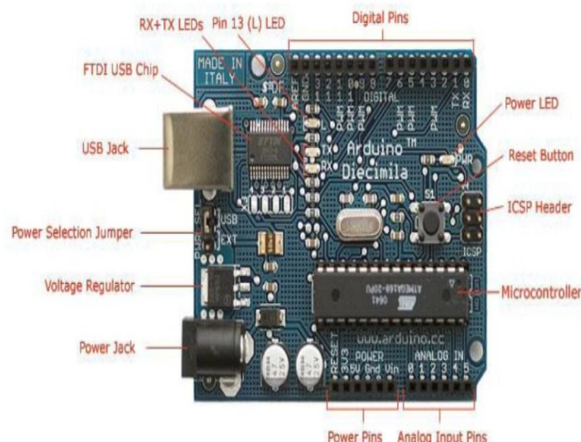
Fig 5. ARDUINO Hardware
