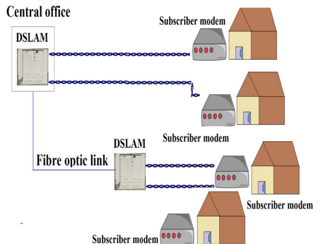
Fig. 4: Hybrid fiber-copper architecture.
