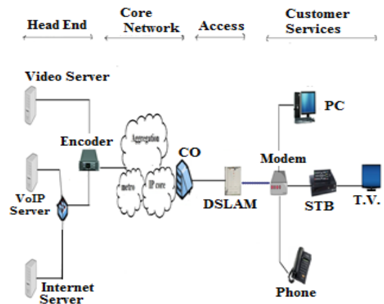
Fig 2: Triple - Play Architecture Overview
