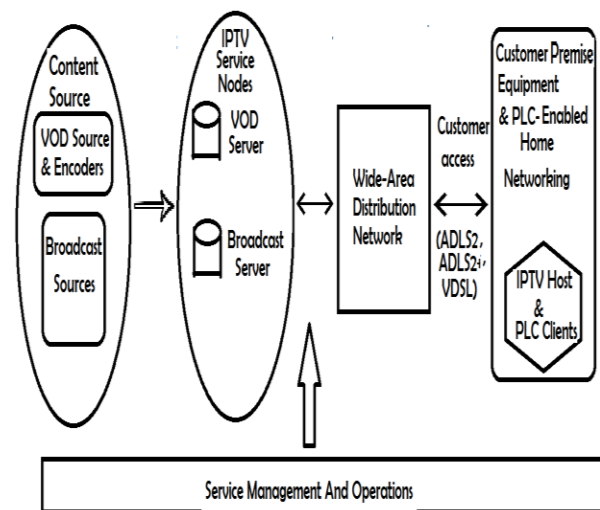
Figure 1: IPTV System Architecture
