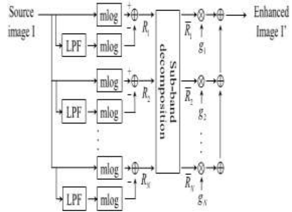
Figure 3: Block diagram of the conventional SD-MSR
