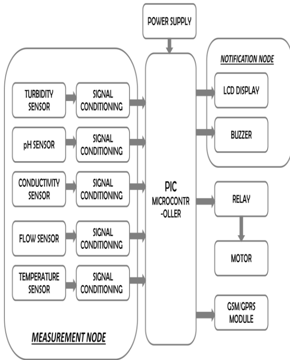
Fig1: Block diagram of measurement and notification node
